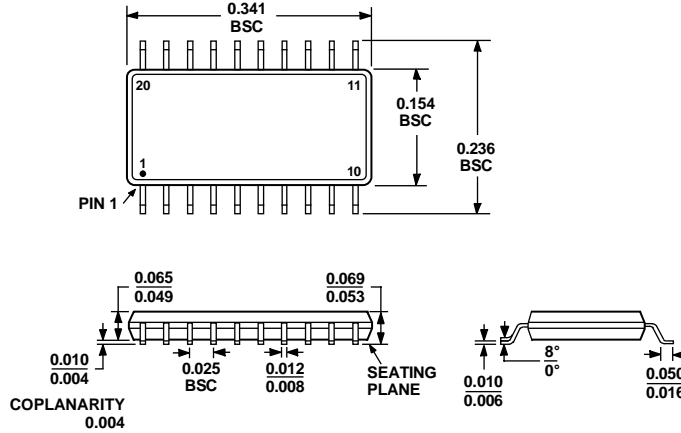
COMPLIANT TO JEDEC STANDARDS MO-137-AD Figure 31. 20-Lead Shrink Small Outline Package [QSOP] (RQ-20) Dimensions shown in inches
